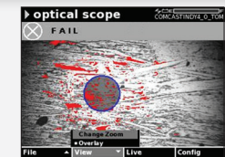
P5000i Fiber Inspection Scope with DSAM
