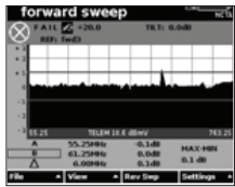
Fwd and Rev Sweep
