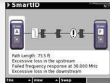
Fault Identification and Location
