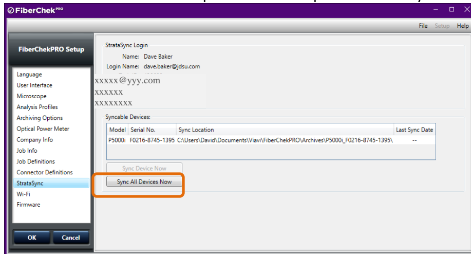
Figure 7: Sync All Devices Now.
