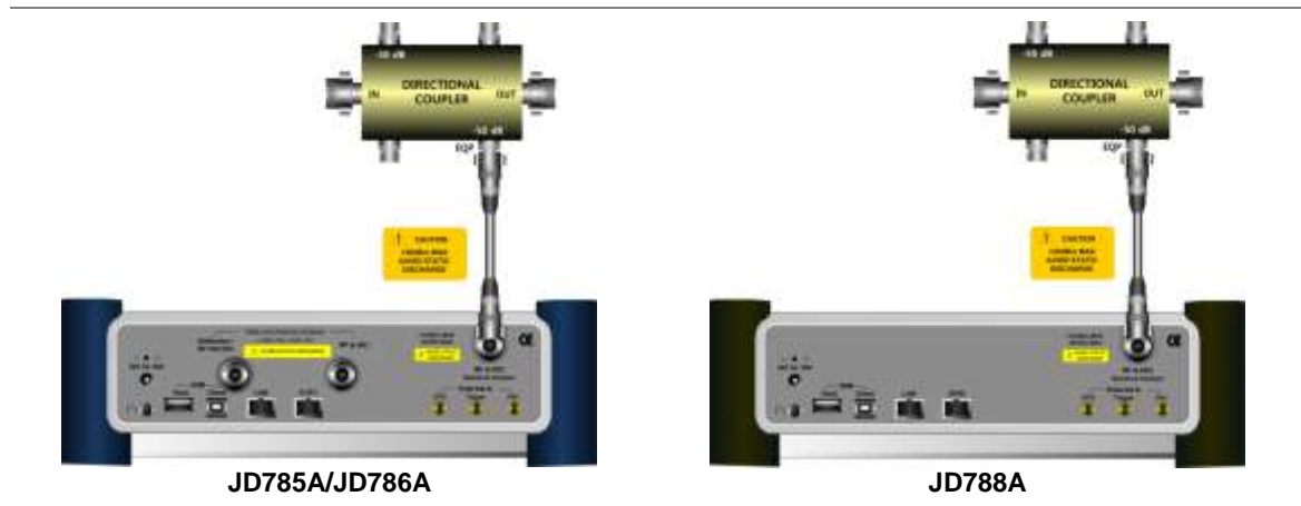
Figure 213 Indirect connection
