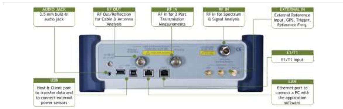
Figure 2 JD785A top panel view
