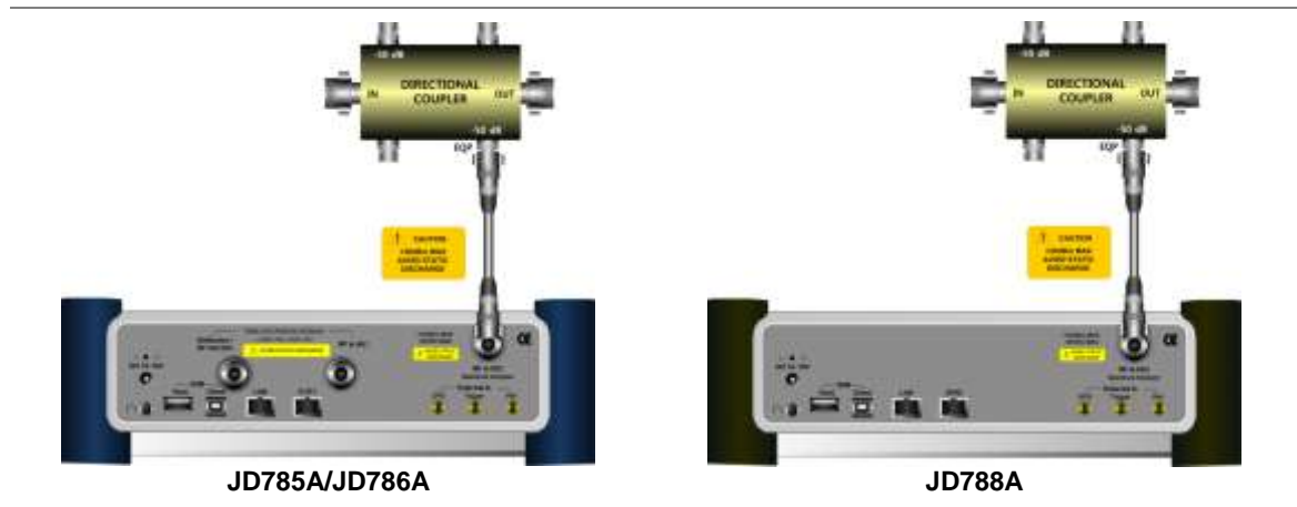
Figure 45 Indirect connection
