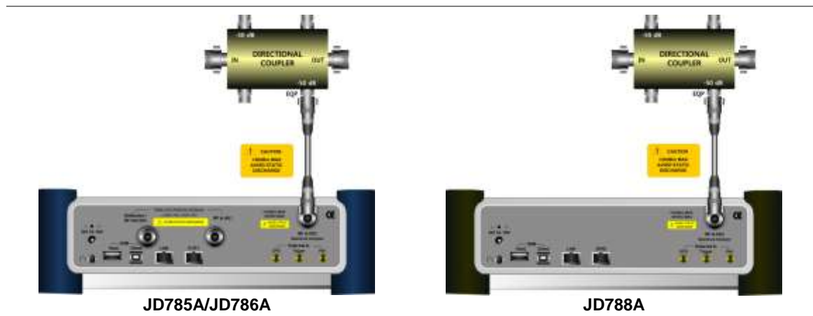
Figure 267 Indirect connection
