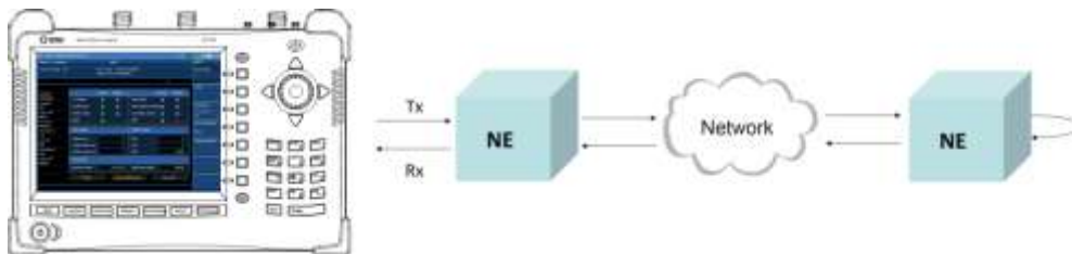
Figure 252 Error injection and measurement connection
