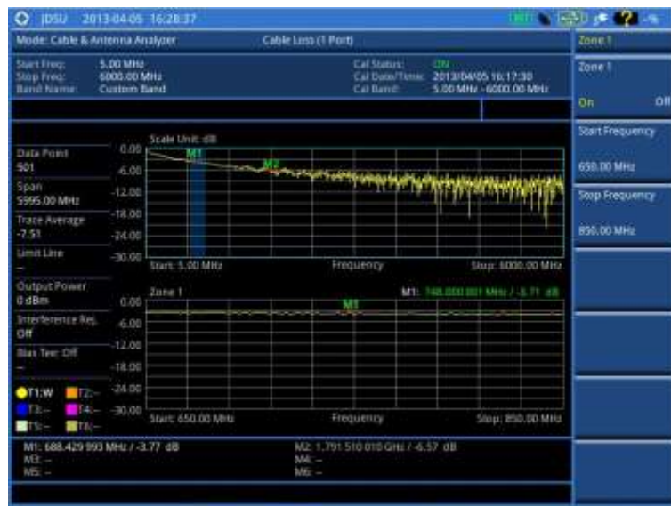
Figure 244 Cable loss (1 port) measurement with the zone enabled
