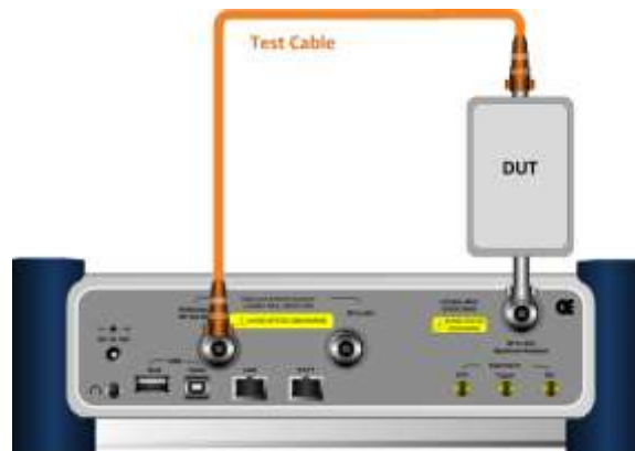
Figure 238 Connection for 2-port scalar measurement
