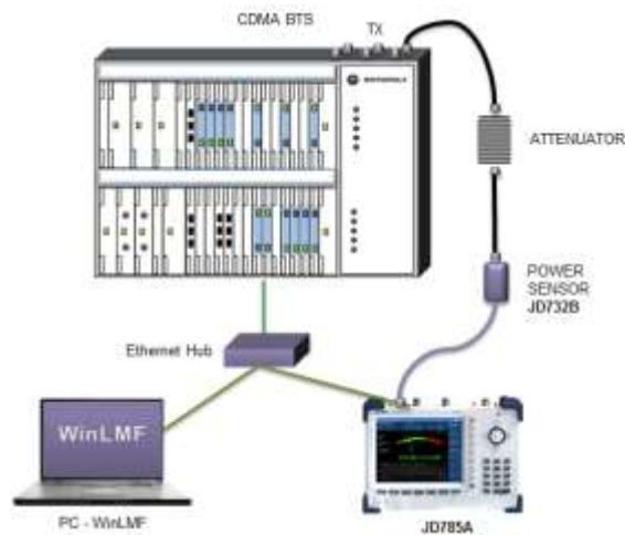
Figure 285 Using external power sensor
