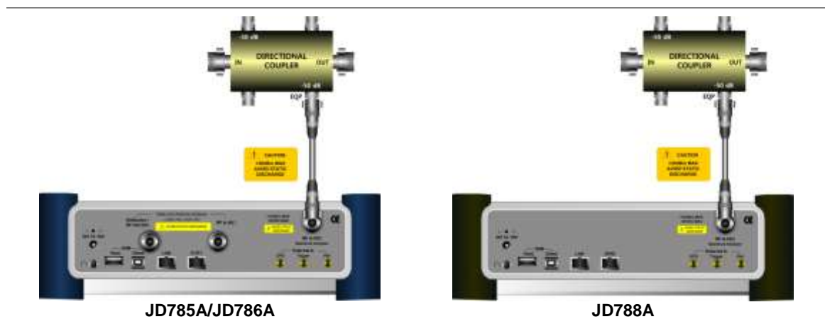
Figure 105 Indirect connection
