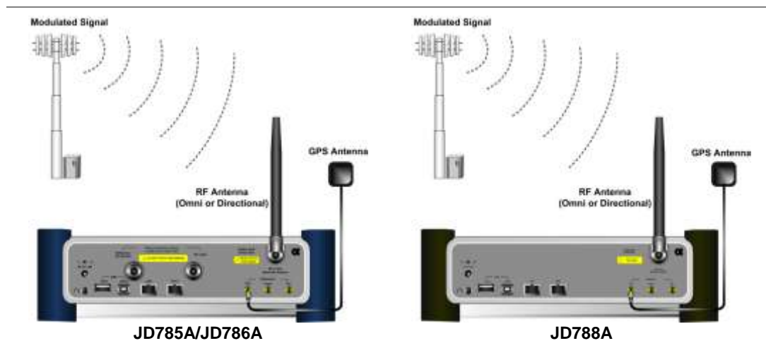
Figure 106 OTA connection
