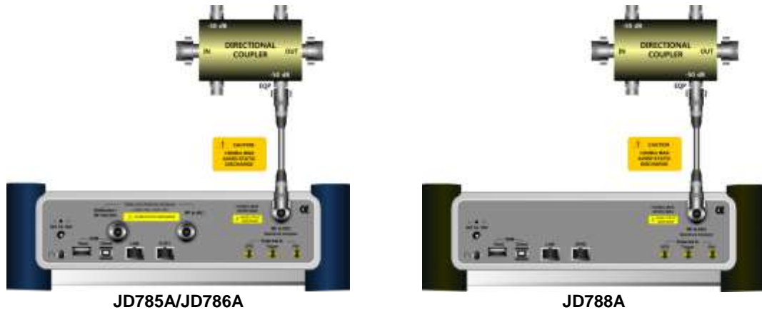
Figure 140 Indirect connection
