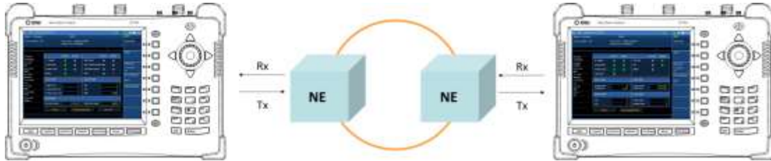
Figure 251 Loop-back connection
