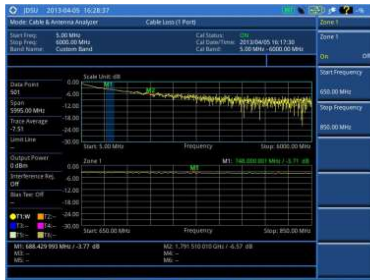
Figure 246 Cable loss (1 port) measurement with zoom
