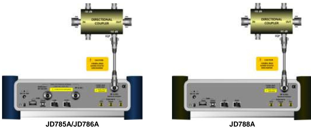
Figure 274 Indirect connection
