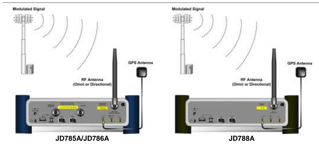
Figure 214 OTA connection
