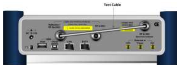
Figure 234 Connection for 2-port calibration in scalar measurement
