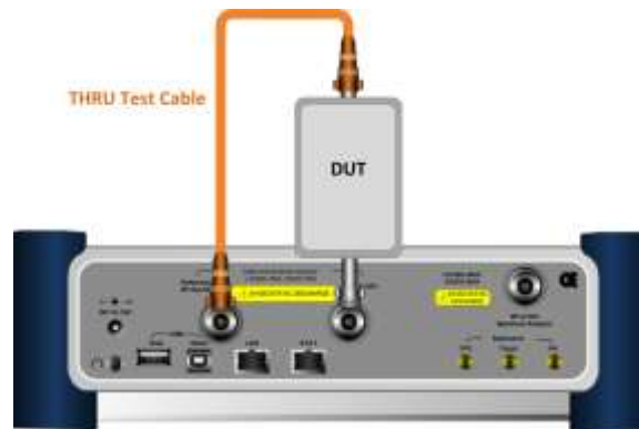
Figure 237 Connection for 2-port vector measurement
