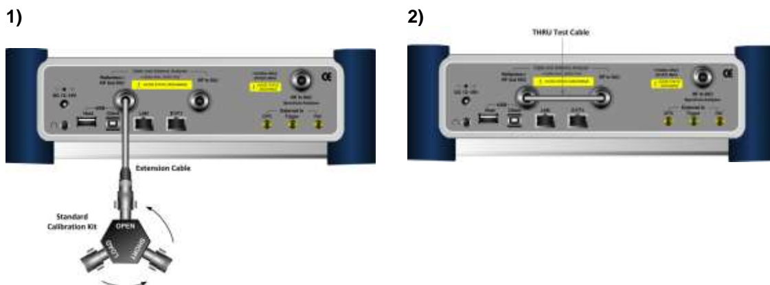
Figure 233 Connection for 2-port calibration in vector measurement
