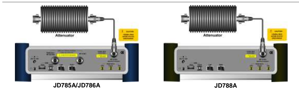
Figure 266 Direct connection
