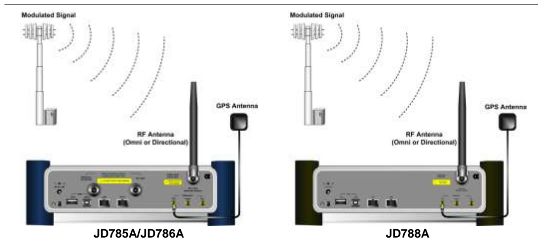
Figure 164 OTA connection
