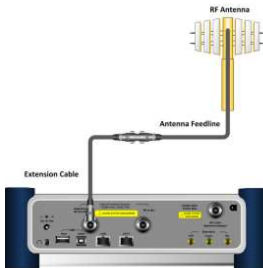
Figure 235 Connection for reflection measurement
