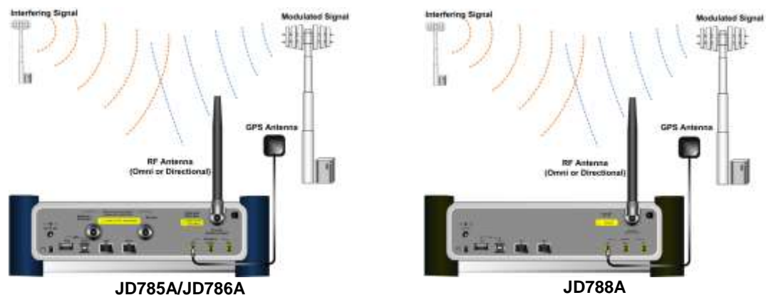
Figure 21 Interference measurement connection
