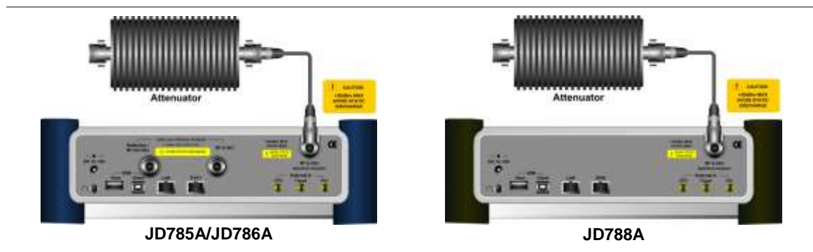
Figure 104 Direct connection
