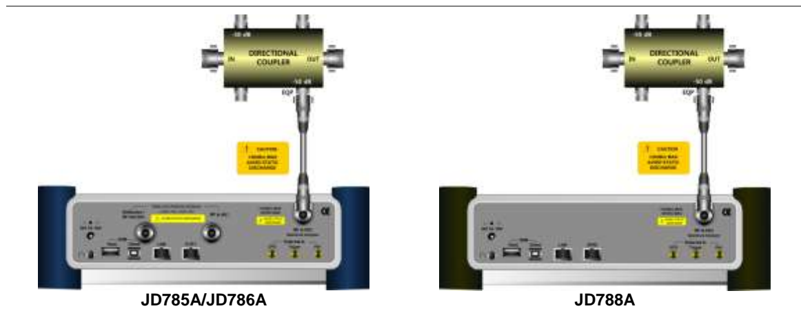
Figure 69 Indirect connection
