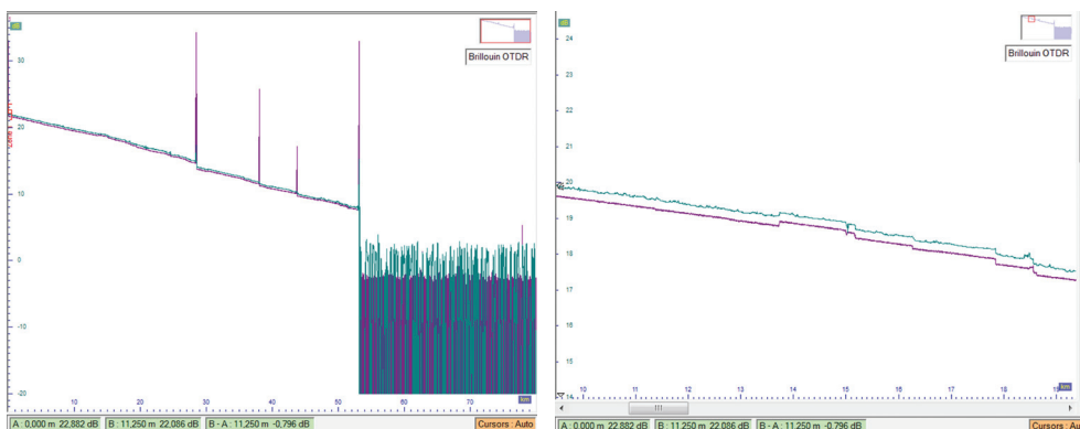
OTDR measurement with zoom on the splices at 15 km.
