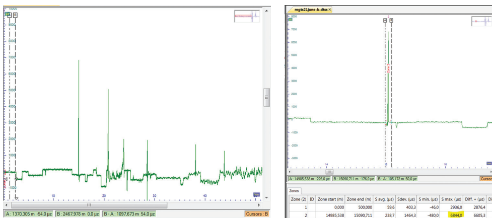
Strain at 15, 21, 24 and 27.5 km along fiber with zoom on strain peak at 15 km.
