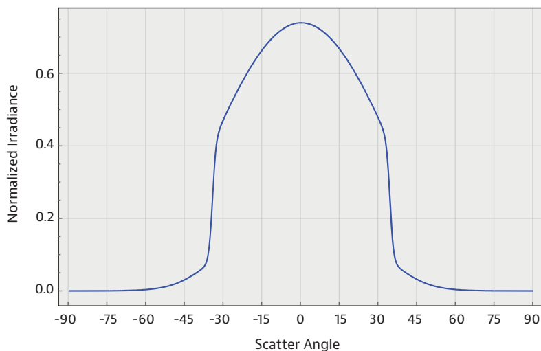
Figure 7. Irradiance Distribution for EDC-60 Engineered Diffuser
