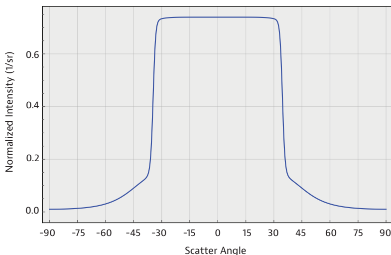
Figure 6. Intensity Distribution for EDC-60 Engineered Diffuser
