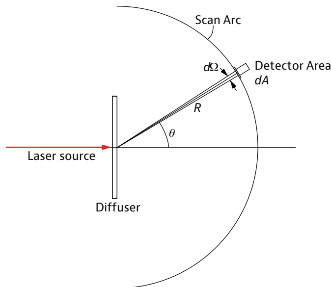
Figure 3. Principle of measurement of intensity
