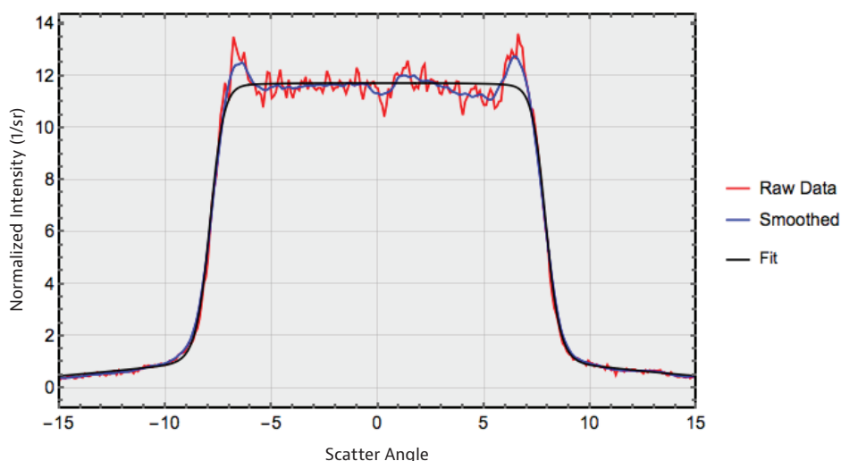
Figure 4. Intensity Distribution for EDC-15 Engineered Diffuser
