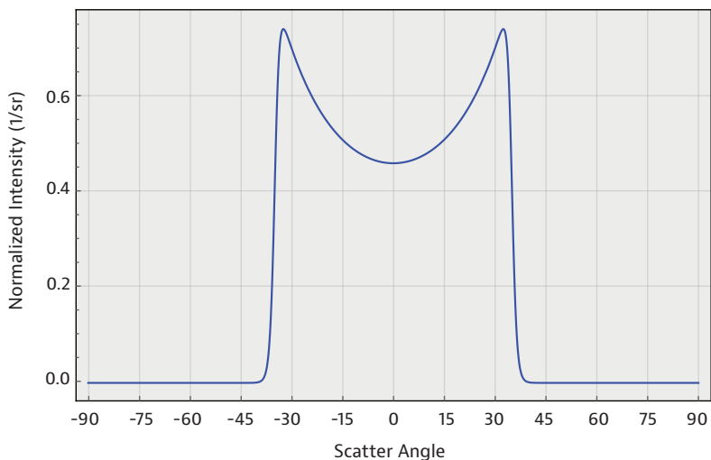
Figure 9. Intensity Distribution for Uniform Irradiance
