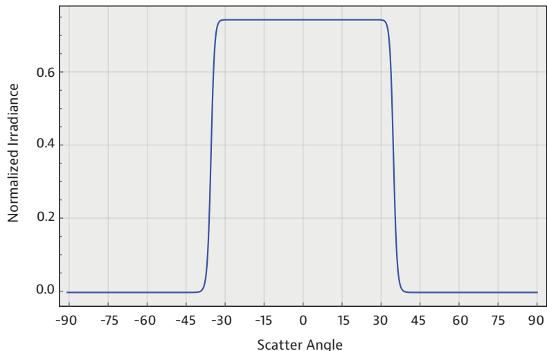
Figure 8. Uniform Irradiance Distribution
