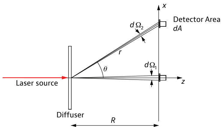
Figure 5. Principle of measurement of irradiance
