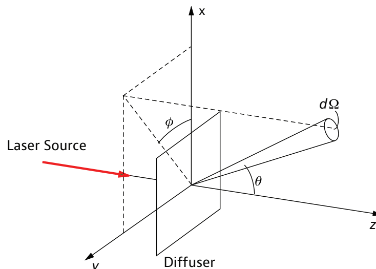
Figure 1. Radiant intensity as a function of scattering angles
